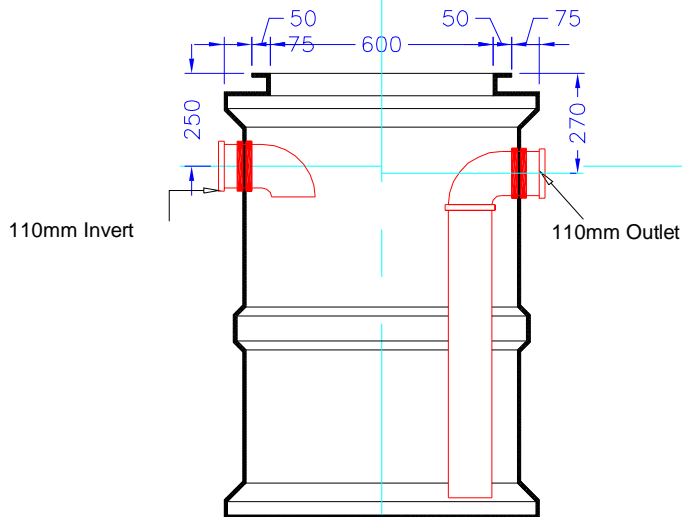
Section Through.
