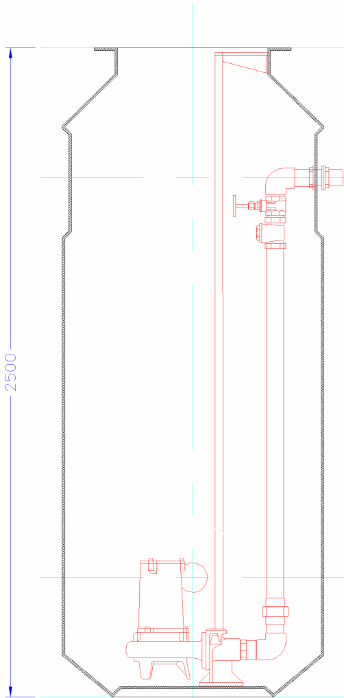
Section Through.
